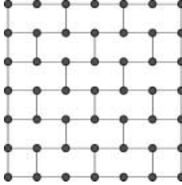
FIG. 6. The grid H_7 .
