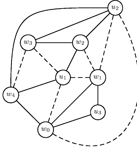
FIG. 9. Vertex u_1 is bad with respect to the cycle C = w_0, w_1, w_2, w_3, w_4 . Vertex u_2 is neutral as it can only be saturated by w_3 . Vertex u_3 is good as it is saturated by the \oplus -assistant w_1 and the \ominus -assistant w_0 . Only the relevant edges are shown.
